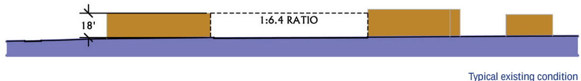
Figure 25: Typical Cross Section through Central Avenue Corridor
