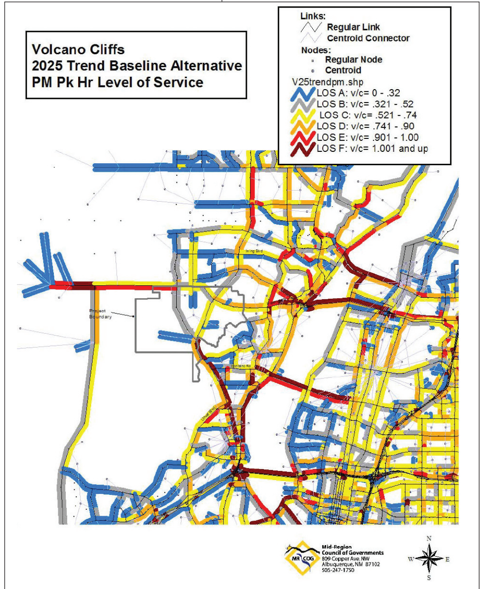
Exhibit 17 Volcano Cliffs 2025 Trend Baseline Alternative PM Peak Hour Level of Service
